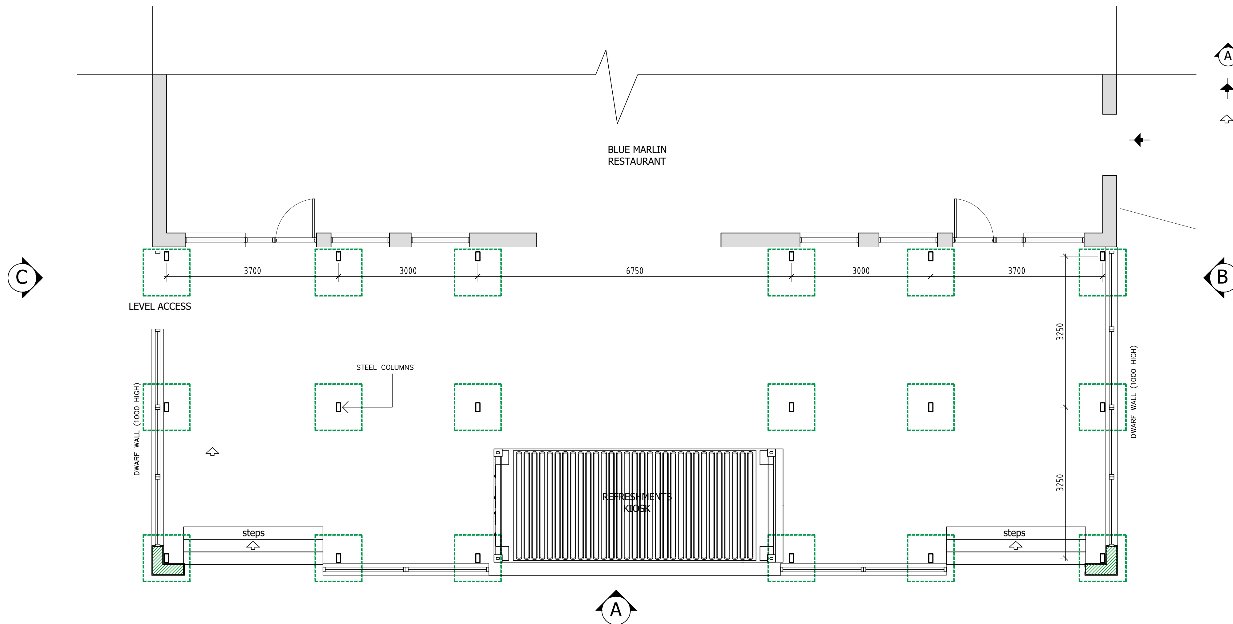
PROPOSED FLOOR LEVEL PLAN 1:50
